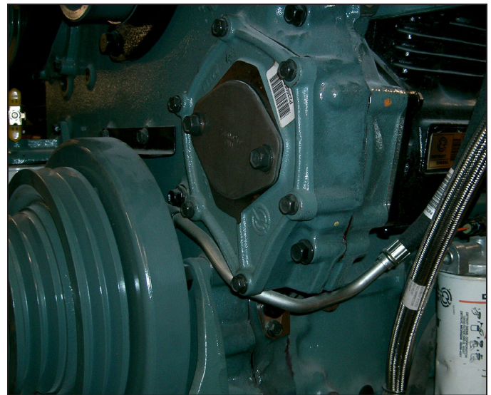
Figure 8 – Coolant Routing (Diesel Engines)
